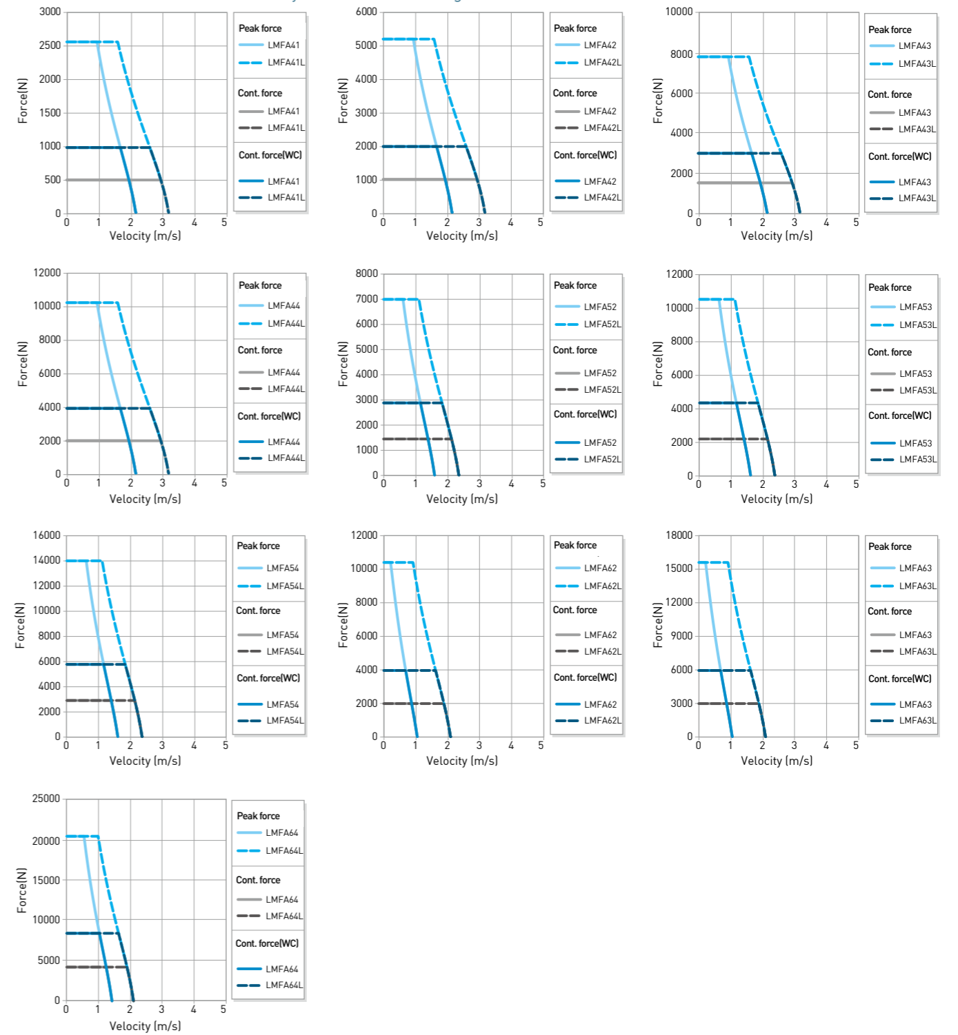
■ Force and velocity curve (DC bus voltage = 325 V DC )
