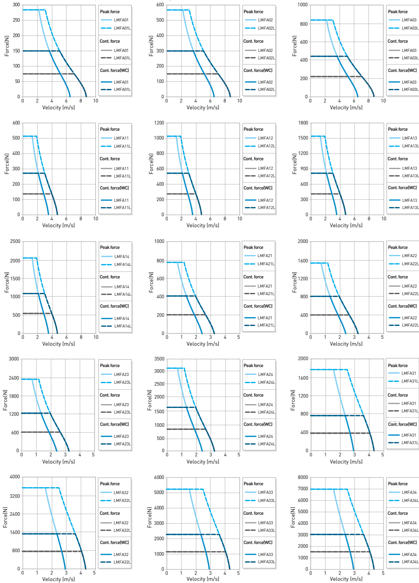
■ Force and velocity curve (DC bus voltage = 325 V DC )
