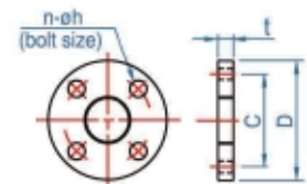
FLANGE DIMENSIONS
