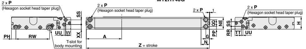
T-slot for body mounting
