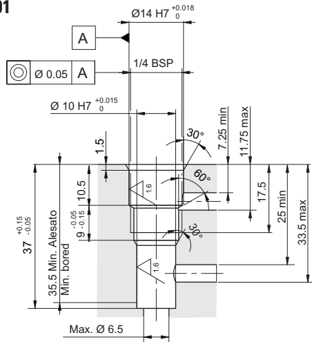
CA012001 1/4 BSP
