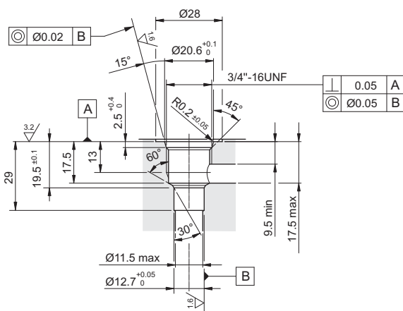
CD018006 3/4 16UNF
