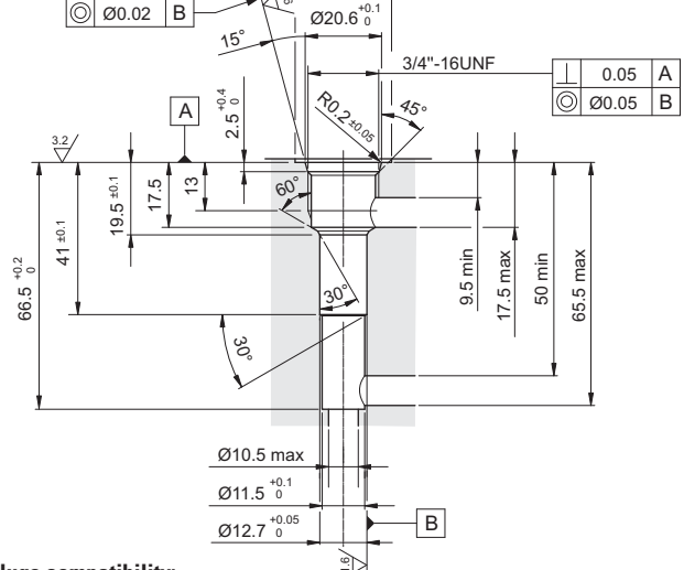
CD018009 3/4 16UNF
