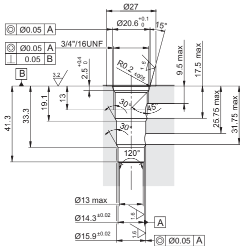
CD018003 3/4 16UNF
