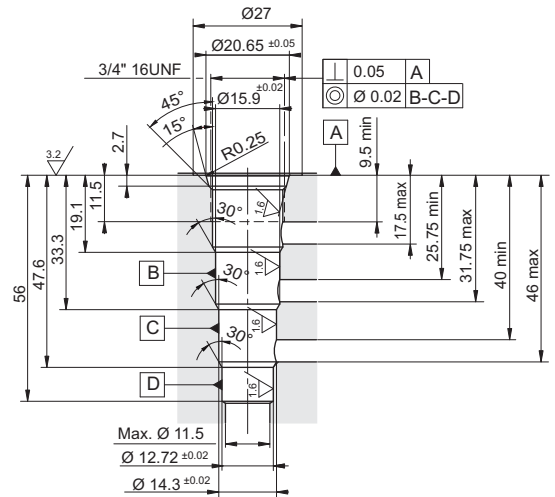
CD018001 3/4 16UNF
