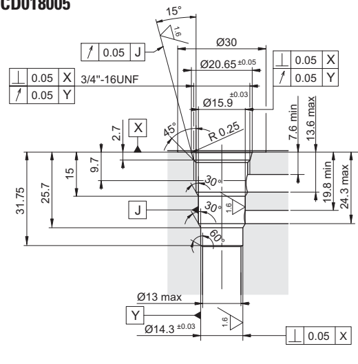
CD018005 3/4 16UNF
