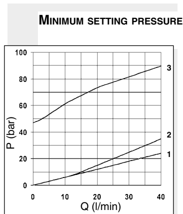
Curves n° 1 - 2 - 3 = setting ranges
